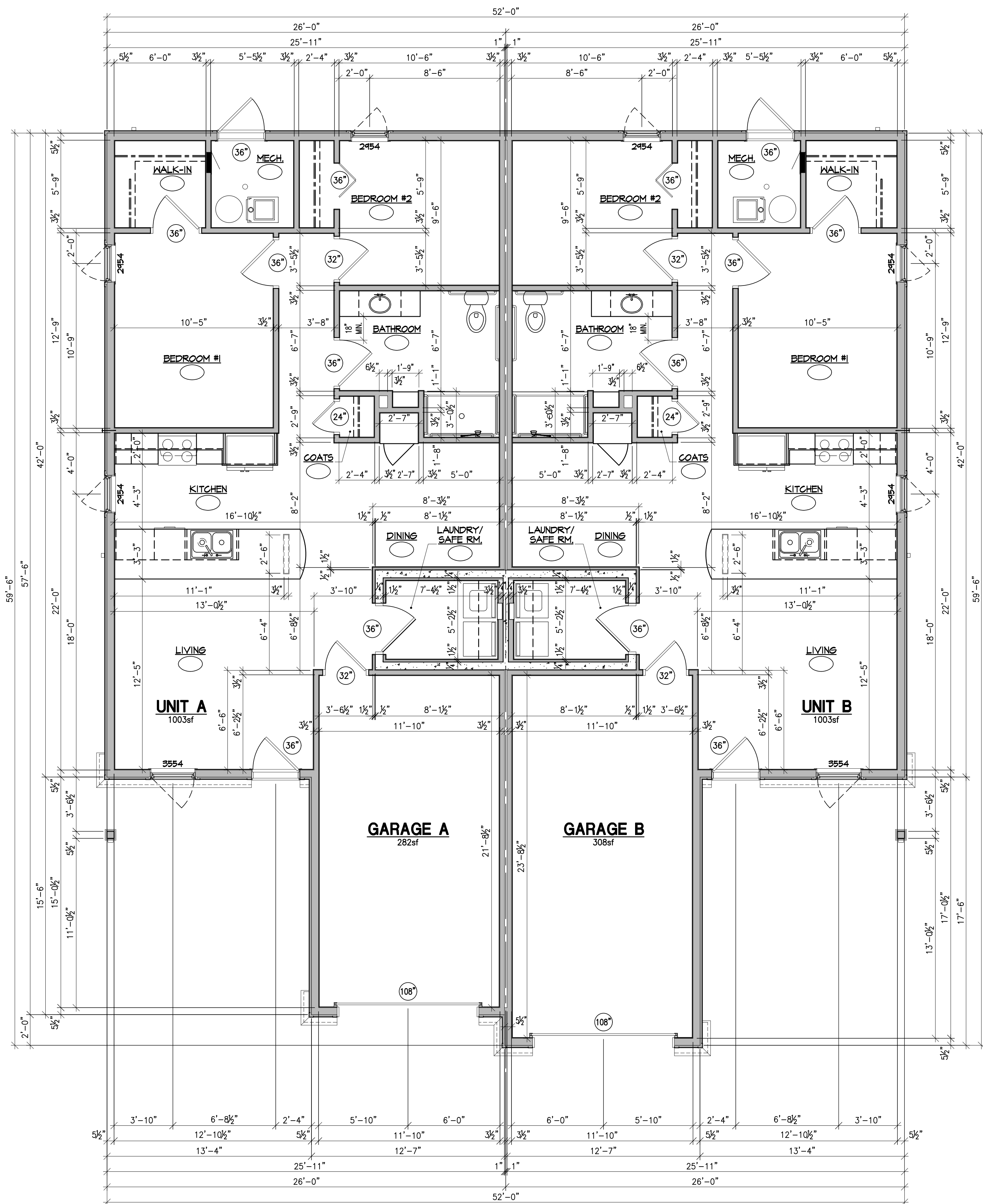
TYPICAL FLOOR PLAN 1/4" = 1'-0" A-FP1SLM
